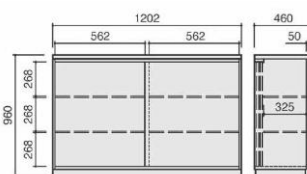
W1200mm
